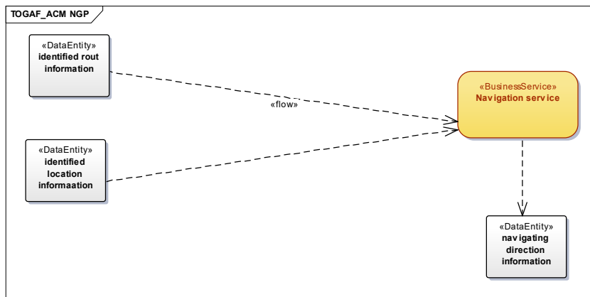
Figure 11 Navigation Business Service to Information Diagram
