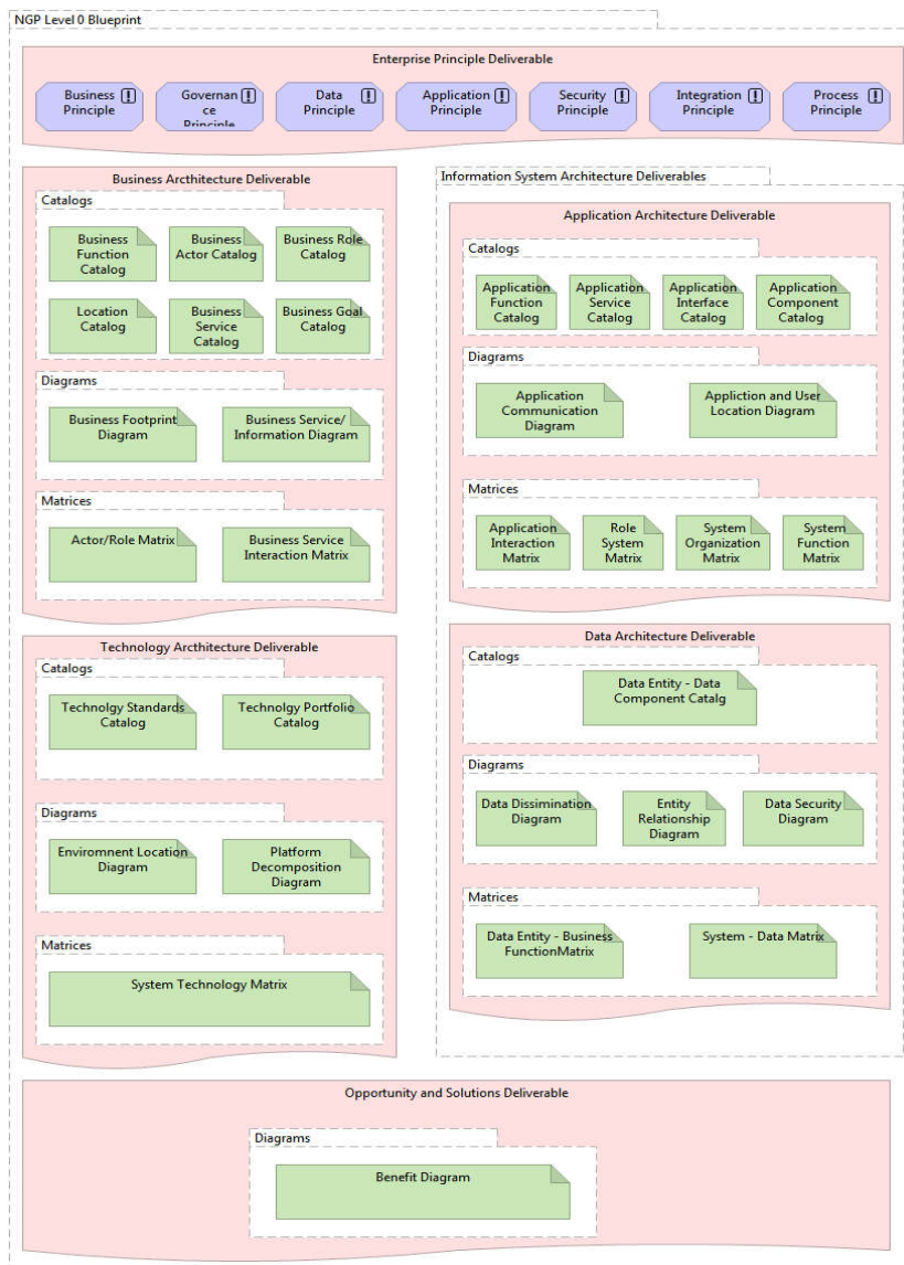
Figure 2. National Geospatial Platform Detail Blueprint (Level 1)
