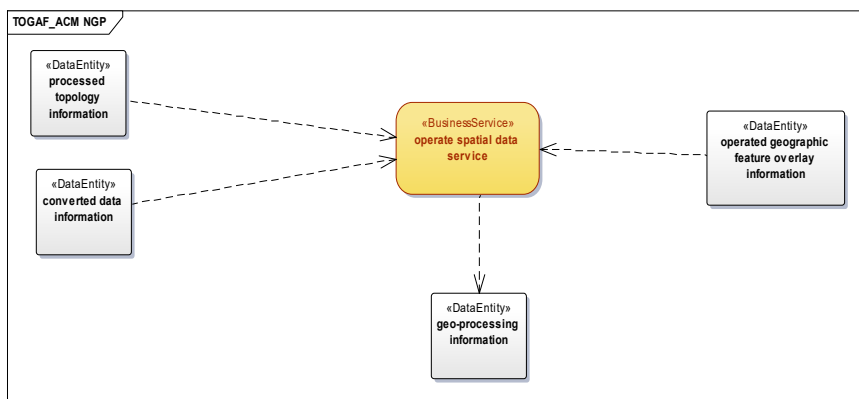
Figure 12. Operation on spatial data Business Service to Information Diagram
