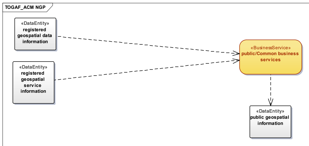
Figure 7. Map Gallery group Business Service to Information Diagram
