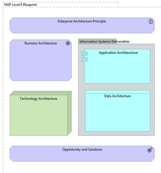
Figure 1. National Geospatial Platform Blueprint (Level 0)
