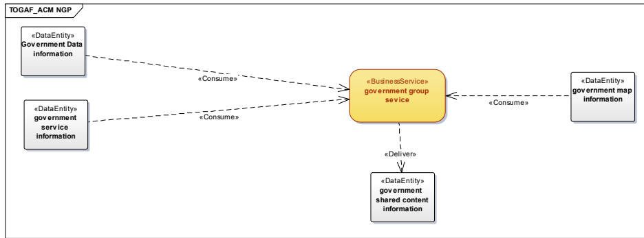
Figure 5. Government group Business Service to Information Diagram
