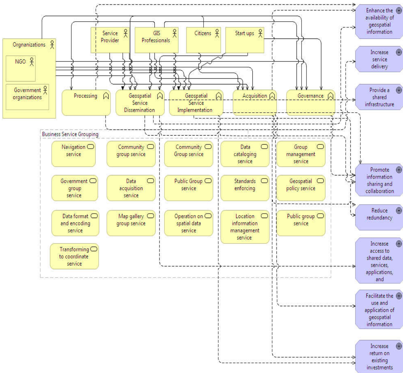
Figure 3. NGP Enterprise Business Footprint Diagram
