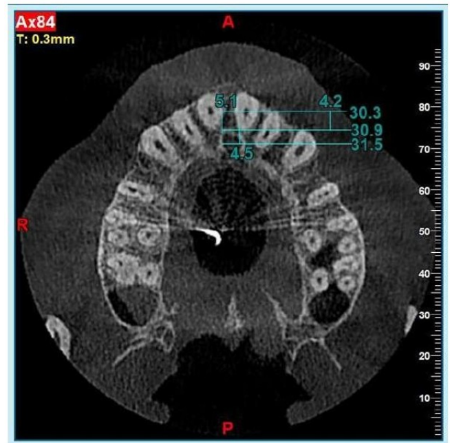
Figure 4: Measurement of Rm-Cat, Rm-Canal, and IC- Root in post treatment CBCT
