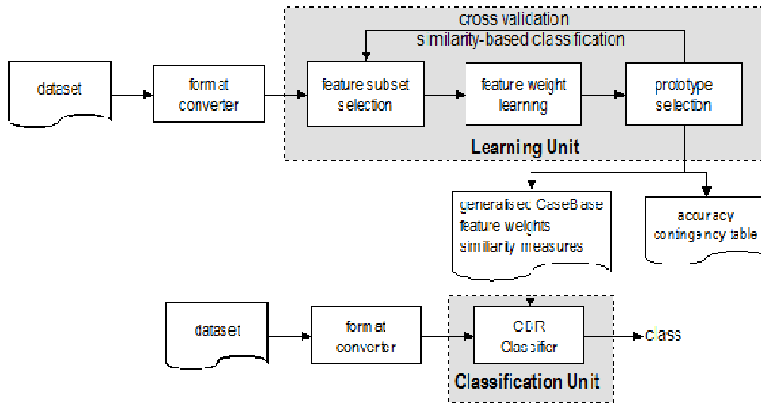
Fig. 5. Prototype-based Classifier
