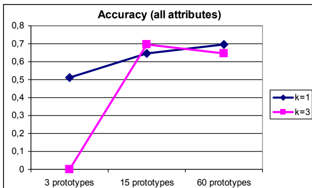
a) Accuracy for different number of prototypes using all attributes
