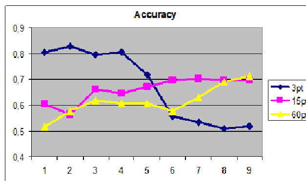
Fig. 7. Accuracy versus Prototypes and for two different feature subset
