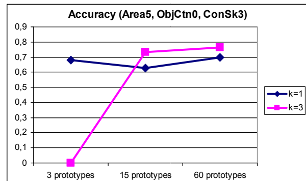
b) Accuracy for different number of prototypes using 3 attributes (Area5, ObjCnt0, ConSk3)
