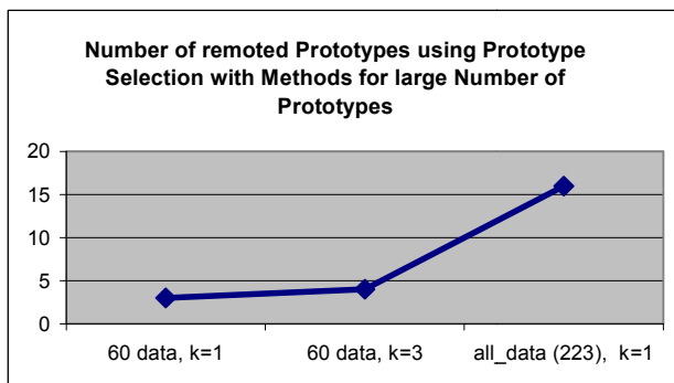
Fig.9. Number of removed Prototypes
