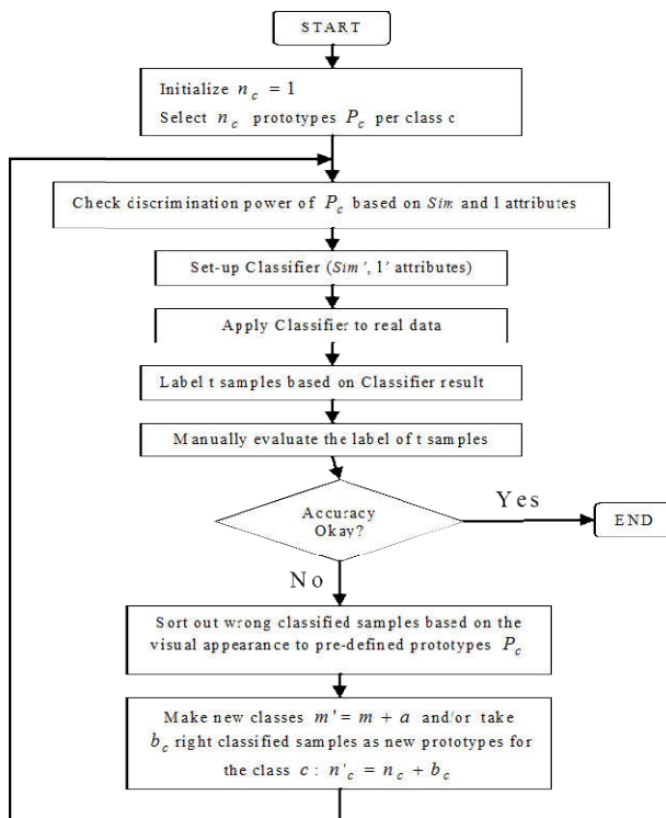
Fig. 3. Methodology for Prototype-based Classification
