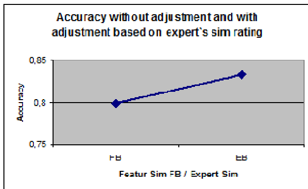
Fig. 8. Accuracy with and without adjustment theory
